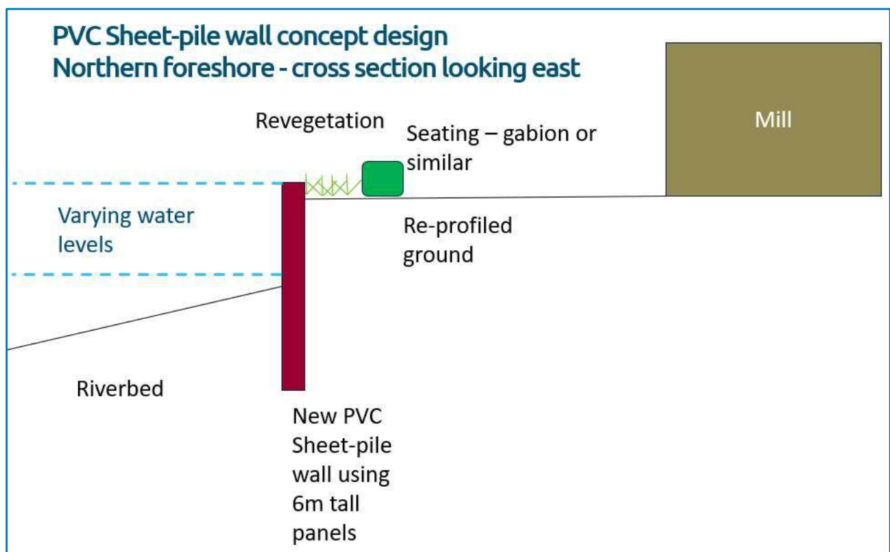
Figure 10-1 Representative cross-section for the PVC sheet pile wall concept design for the Northern foreshore. Areas for revegetation and simple seating are depicted. The seating could provide additional resistance to water flows in high water level events to reduce impacts to the Mill. The area between the seating and the Mill could be used for landscaping and education signage.
