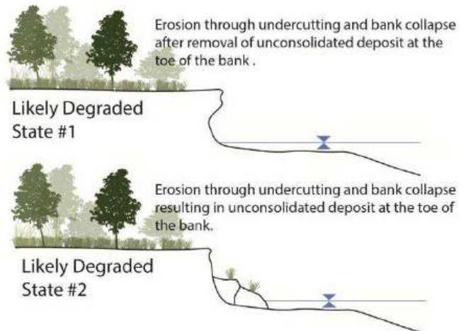
Figure 2-12 Diagram demonstrating how erosion from wave action and boat wash can affect banks.
