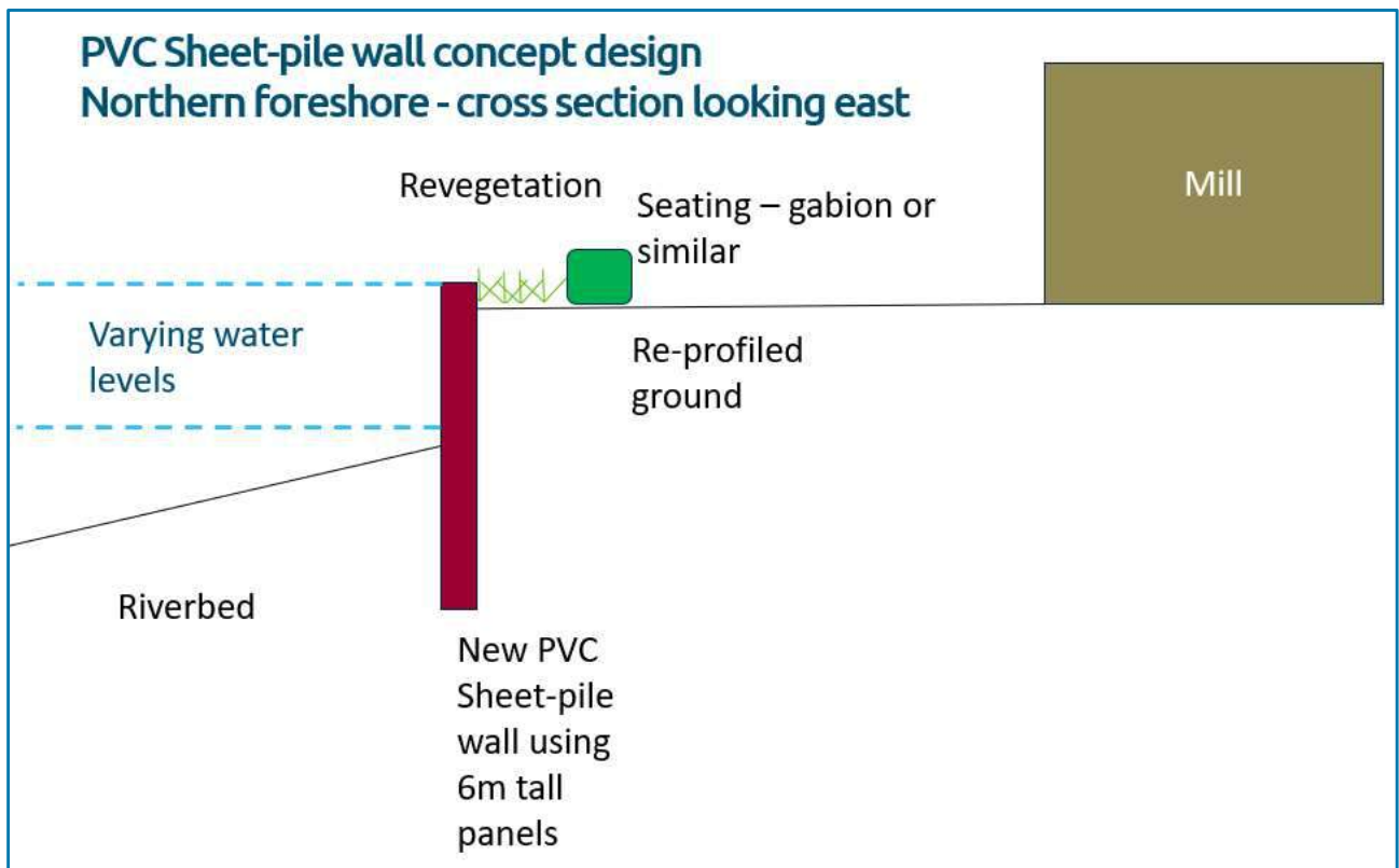
Figure 1-2 PVC sheet pile wall concept design - Northern foreshore – representative cross-section.
