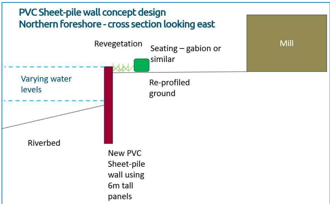
Figure 9-6 Representative cross-section for the PVC sheet pile wall concept design for the Northern foreshore. Areas for revegetation and simple seating are depicted. The seating could provide additional resistance to water flows in high water level events to reduce impacts to the Mill. The area between the seating and the Mill could be used for landscaping and education signage.
