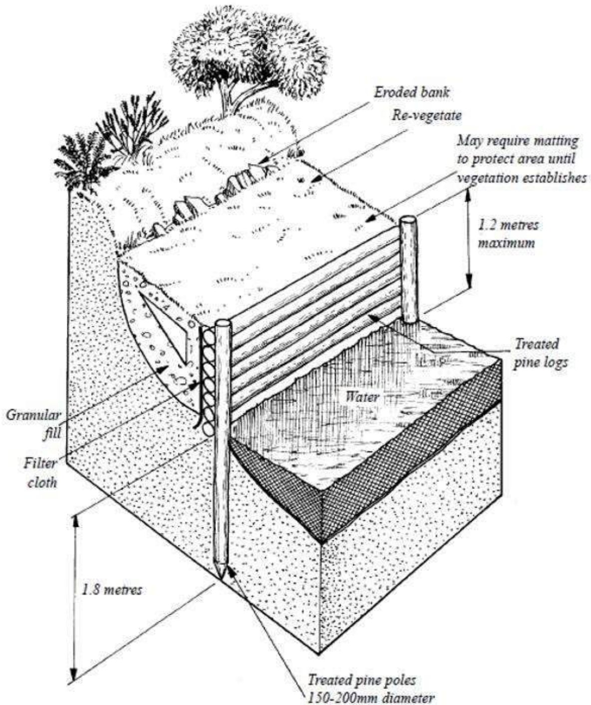
Figure 9-3 Piled log wall (Water and Rivers Commission, 2000)
