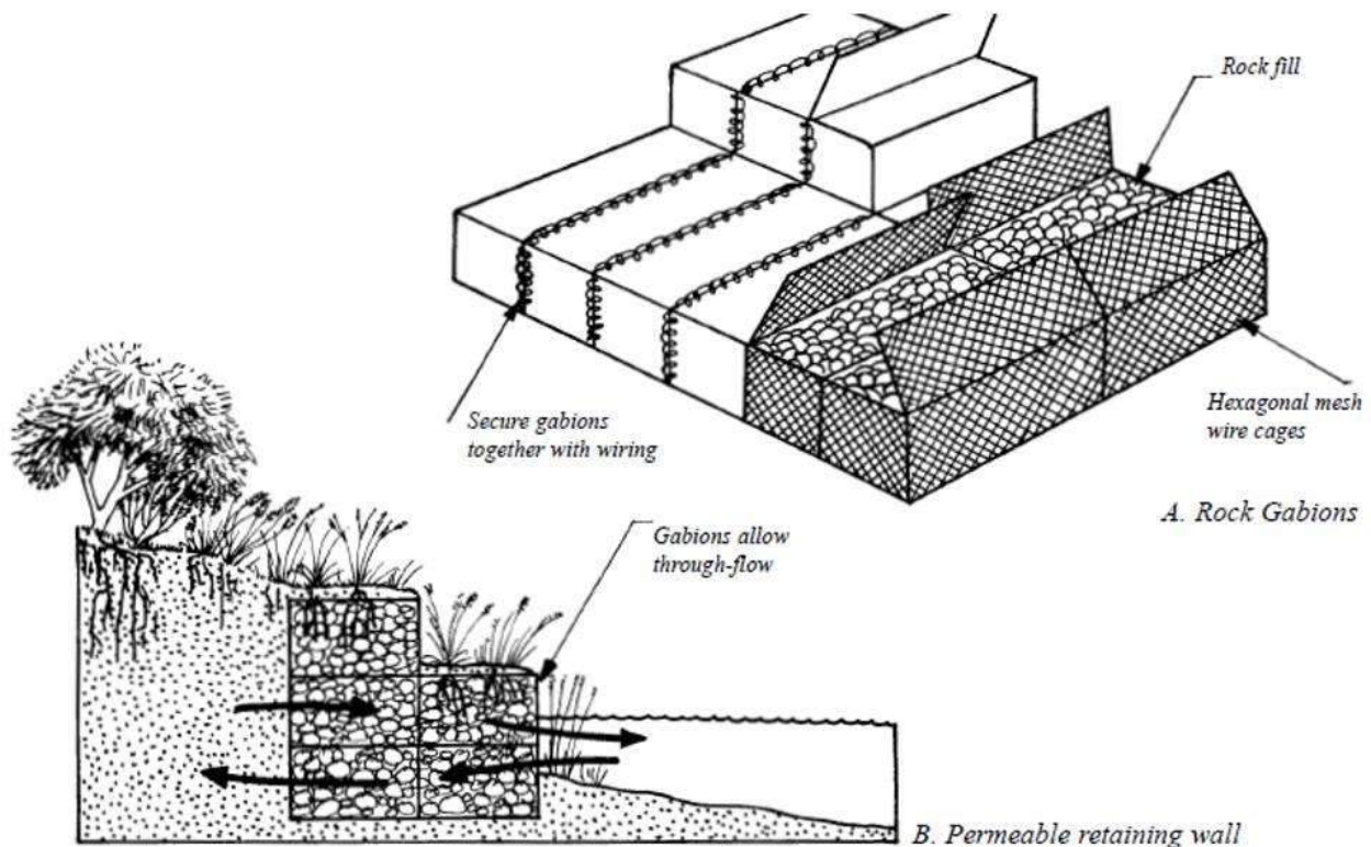
Figure 9-2 Gabion wall (Water and Rivers Commission, 2000)
